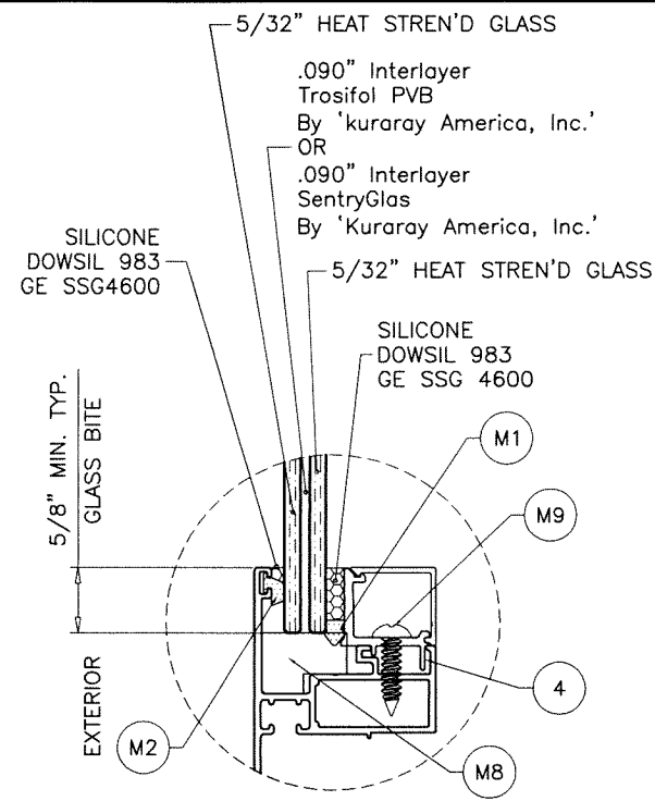
GLASS TYPE 'A' 3/8" OVERALL LAM. GLASS
